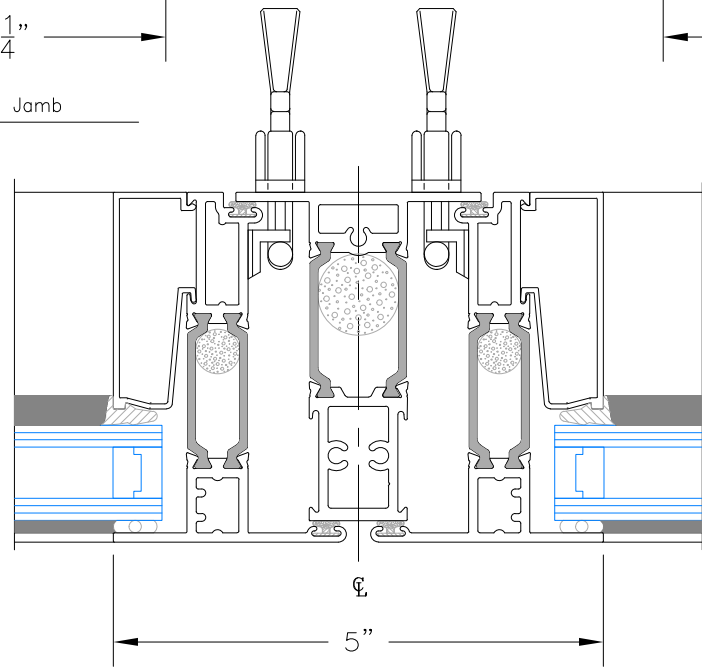
8 Vertical Mullion
