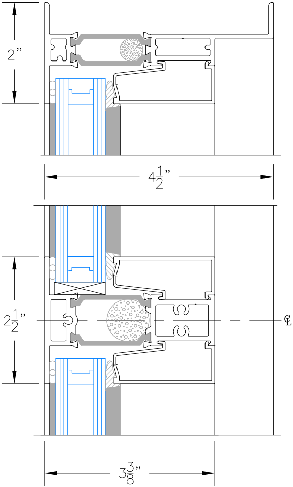
2 Horizontal Mullion
