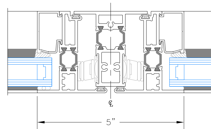
20 Vertical Mullion
