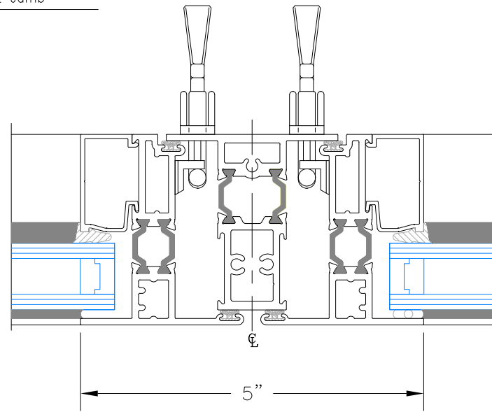
8 Vertical Mullion
