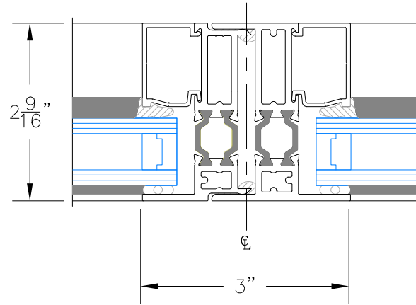
10 Vertical Stack
